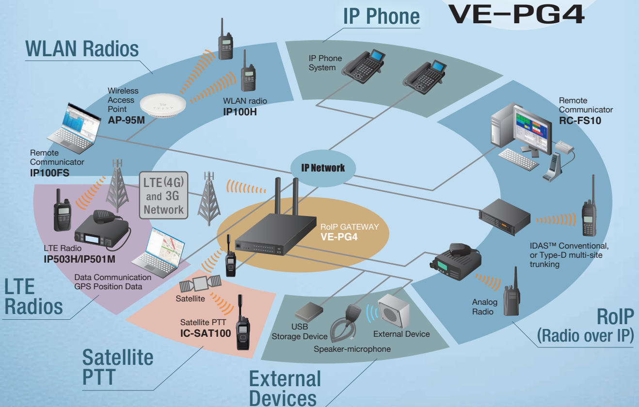
RoIP GATEWAY
